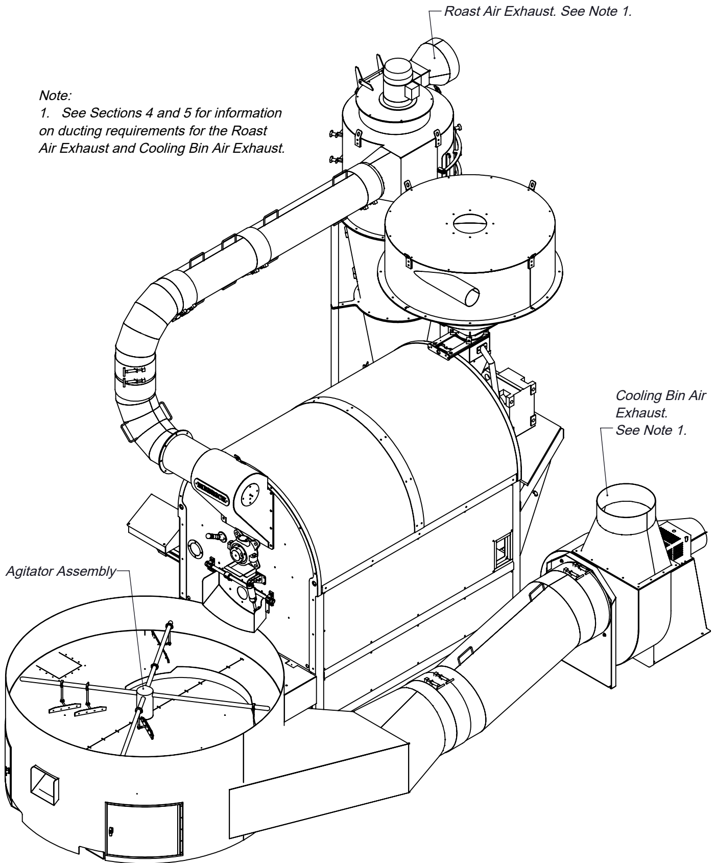
Front Right - Isometric View
